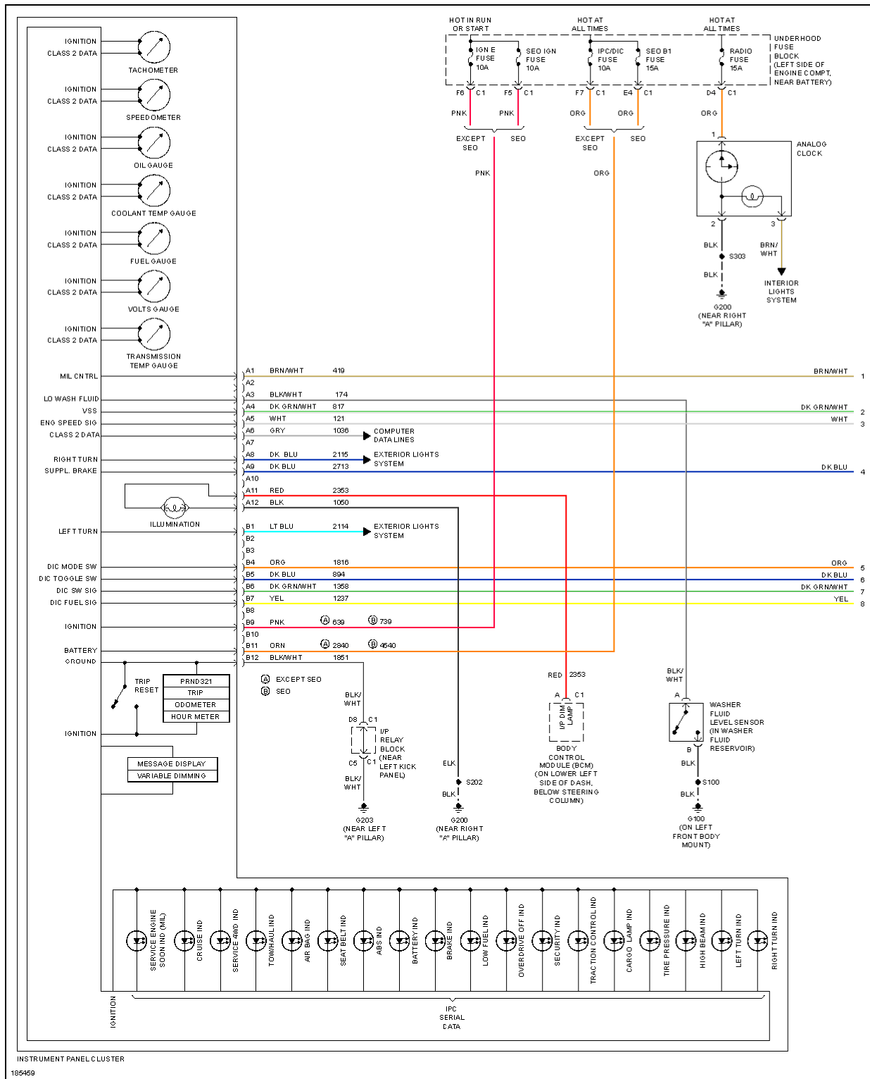
Fig. 49: Instrument Cluster Circuit (1 of 2)
